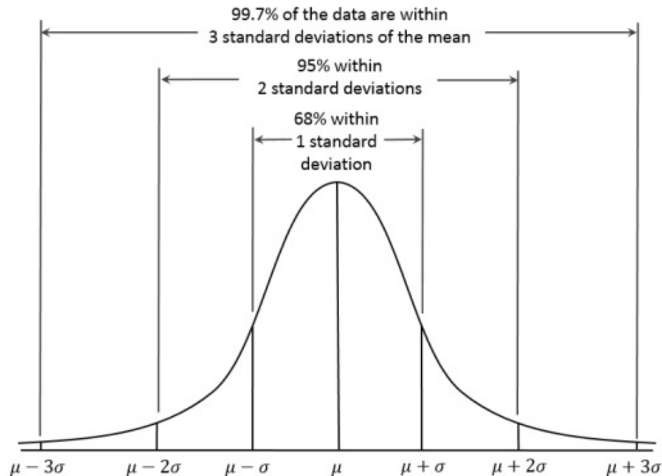
Figure 2-10. Normal curve
